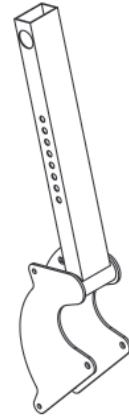
(3) BACK SUPPORT FRAME
