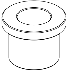
(13) x22 \phi 20 \times \phi 16 \times \phi 10.2 \times 15 Sleeve Spacer
