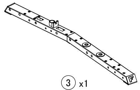
Base Frame - Left
