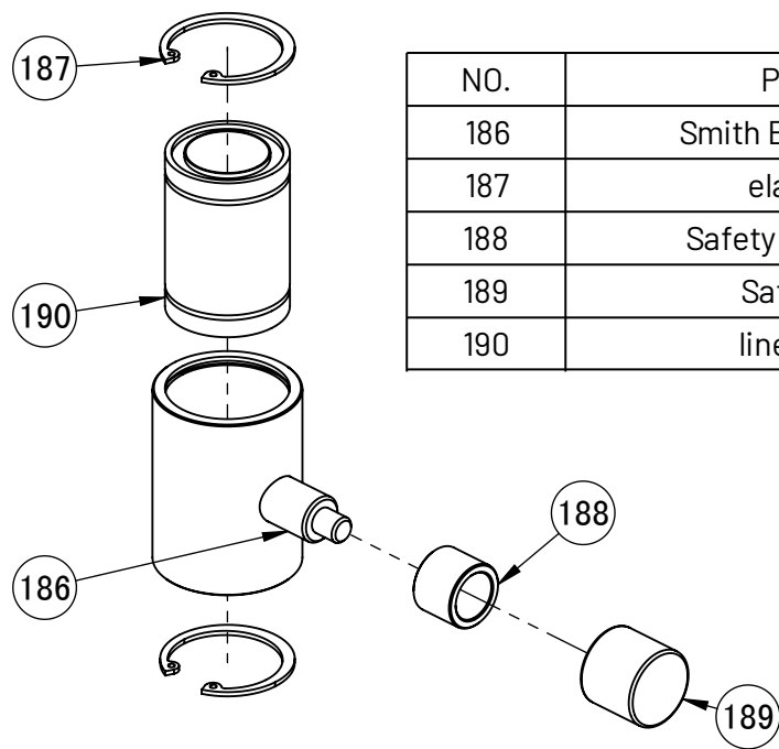
60 x2 Smith Bar Sliding Frame
